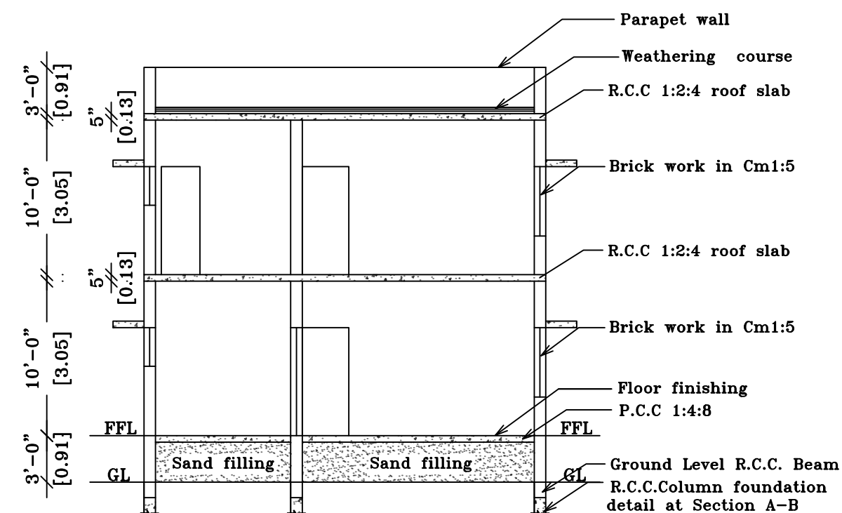
SECTION ON 'SD'
