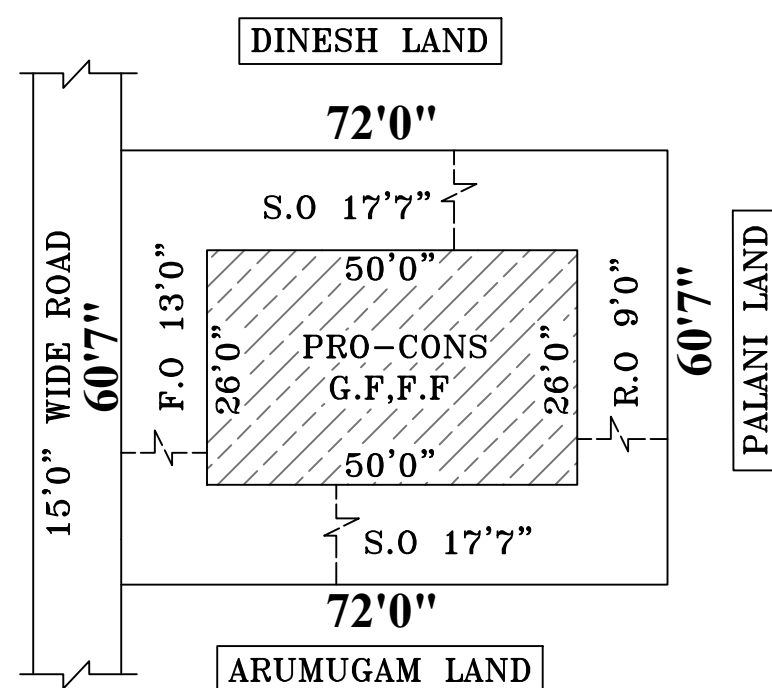
SITE PLAN
