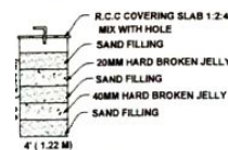
rain Water Harvest Unit Not To Scale
