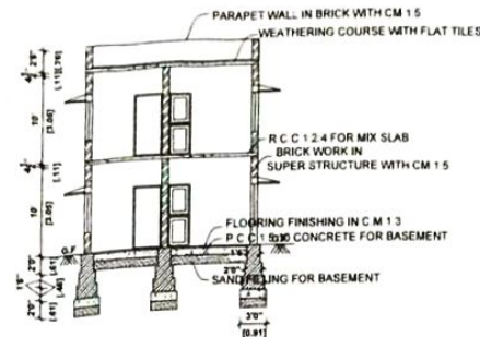
SECTION NO R-S
