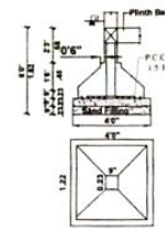
COLUMN DETAIL NOT TO SCALE
