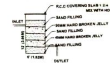
Waste Water Recycle Unit Not To Scale
