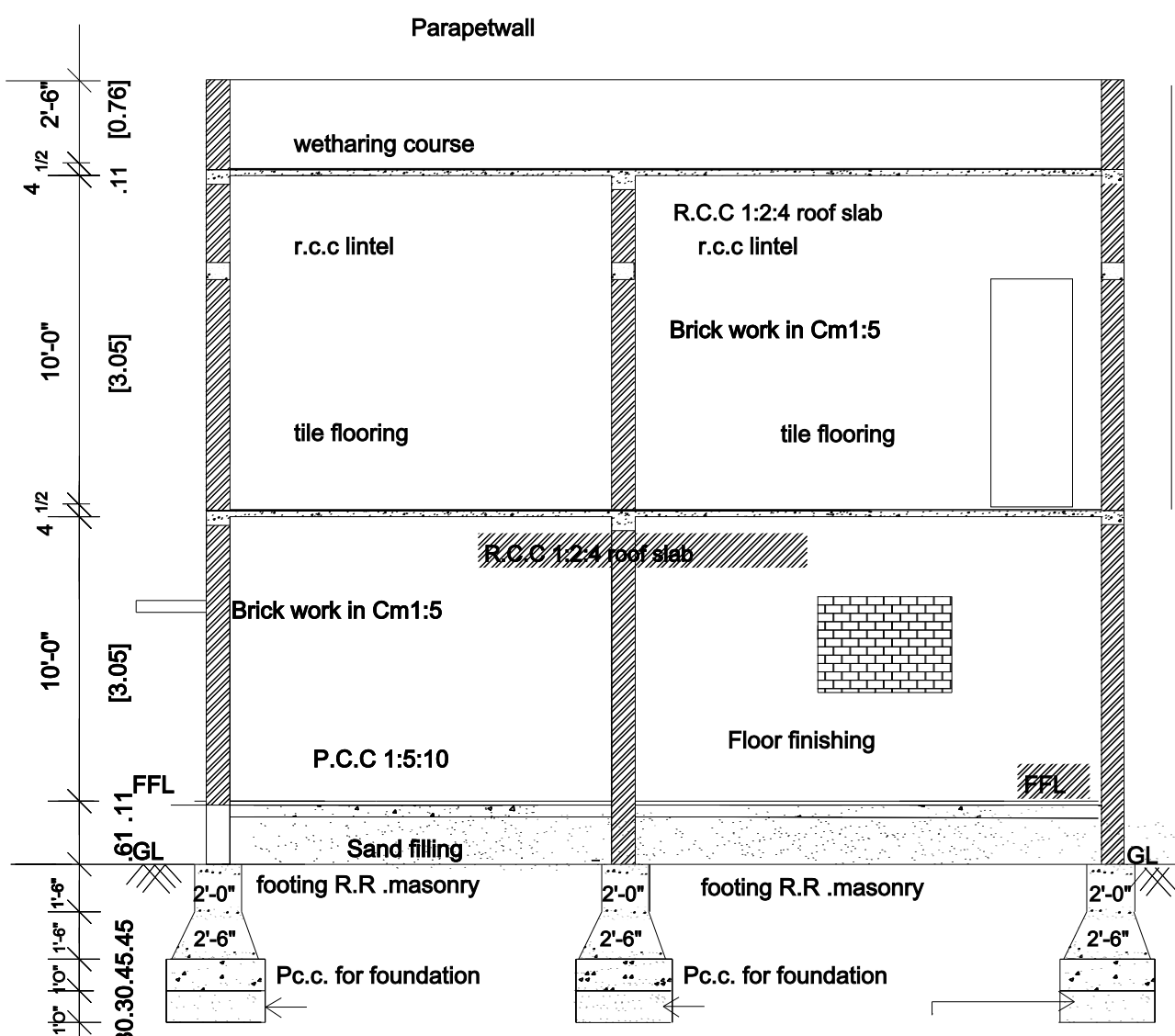
SECTION ON "SB"
