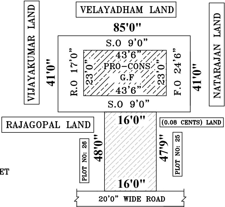
SITE PLAN
