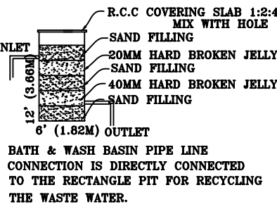
WASTE WATER RECYCLE UNIT
