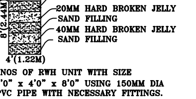
RAIN WATER HARVEST UNIT
