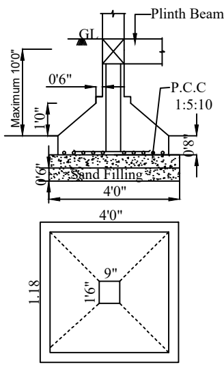
COLUMN DETAIL
