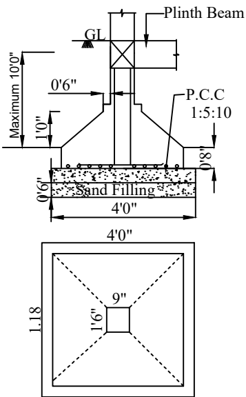
COLUMN DETAIL
