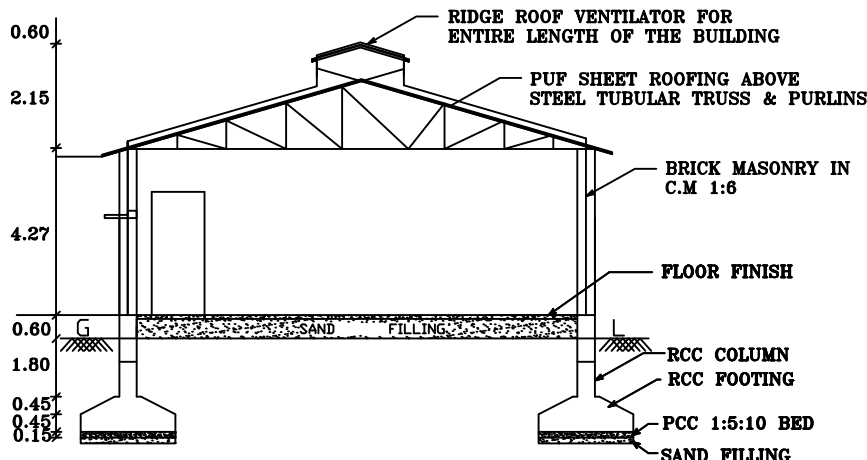
SECTION ON 'SK'
