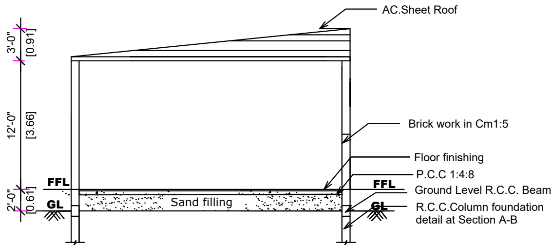
SECTION ON 'RK'
