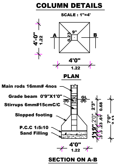
COLUMN DETAILS
