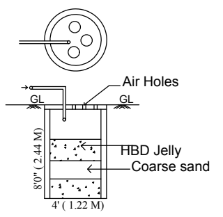
IN WATER HARVESTING TANK DETAIL
