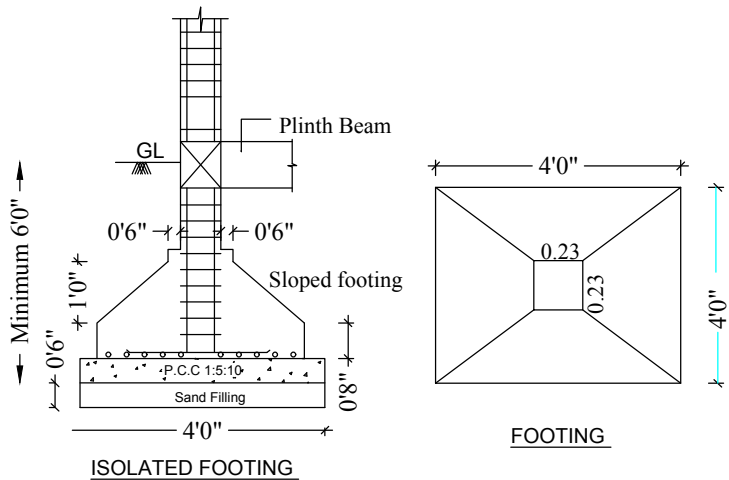
COLUMN DETAILS
