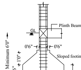
COLUMN DETAILS
