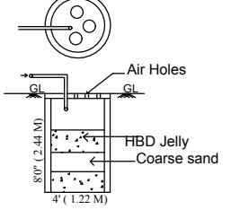
RAIN WATER HARVESTING TANK DETAIL
