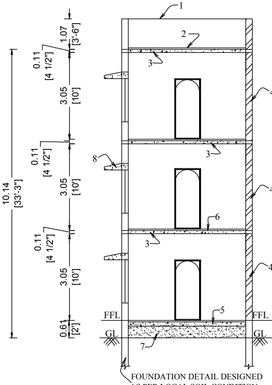
SECTION ON 'J-S'
