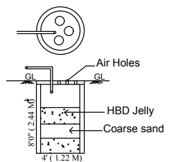
WASTE WATER RECYCLE UNIT
