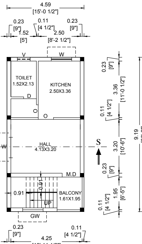
TYPICAL FLOOR PLAN (1st, 2nd FLOOR PLAN)
