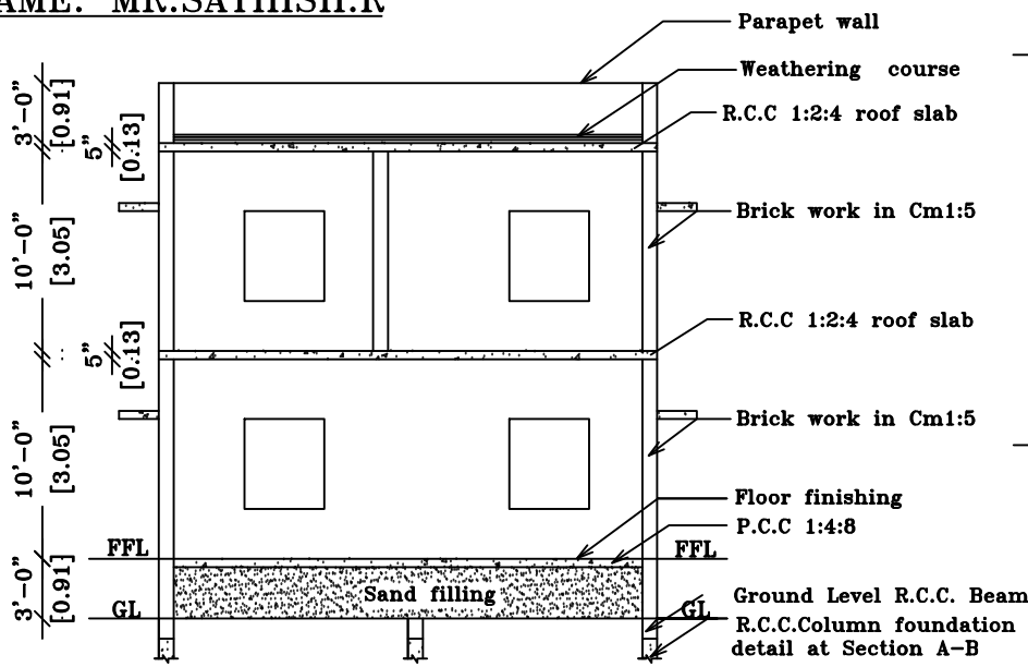
SECTION ON 'SD'
