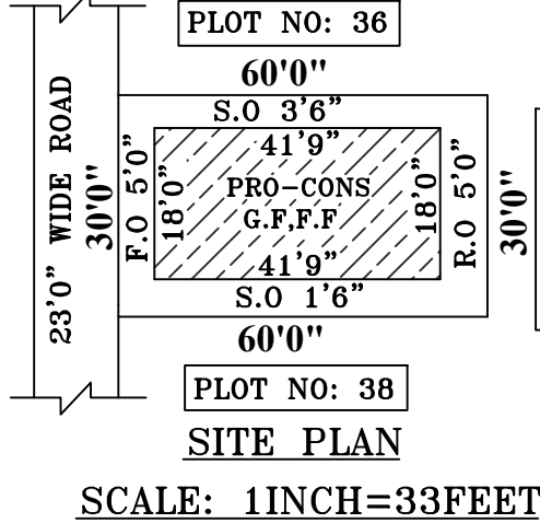
SITE PLAN
