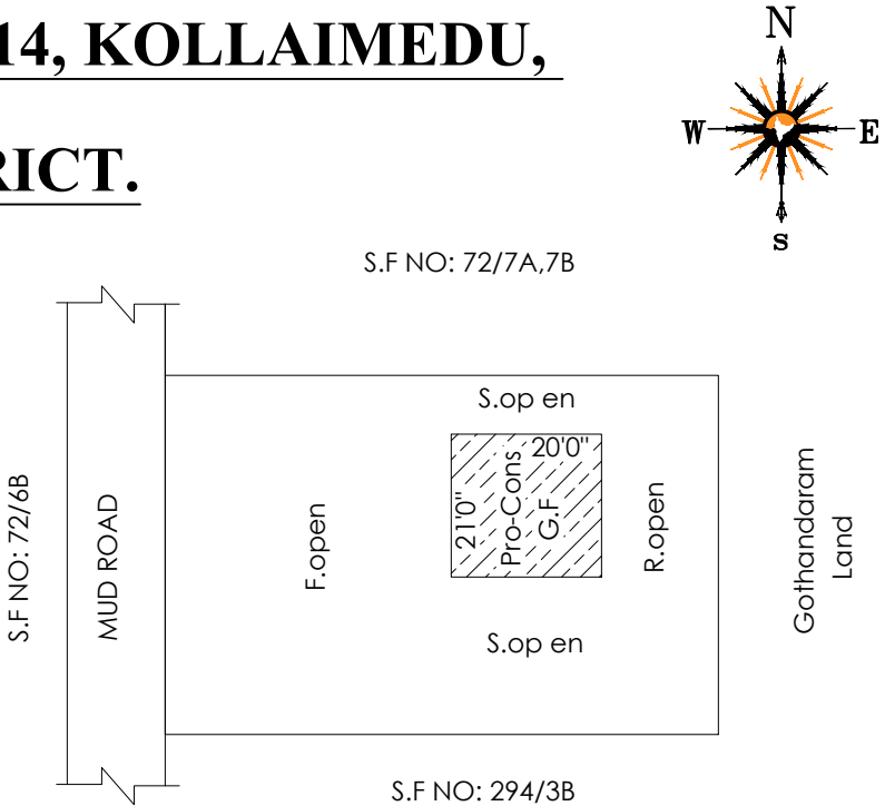
SITE PLAN
