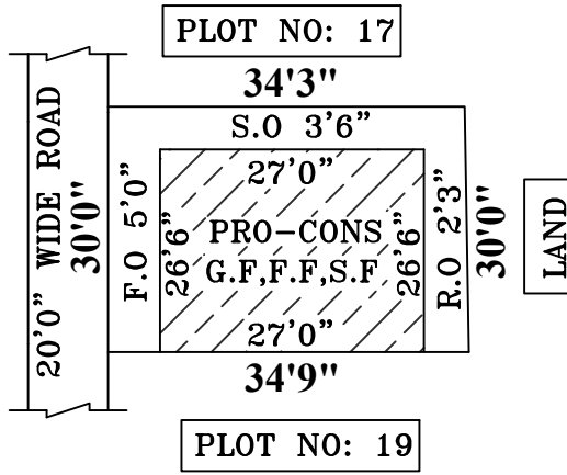
SITE PLAN
