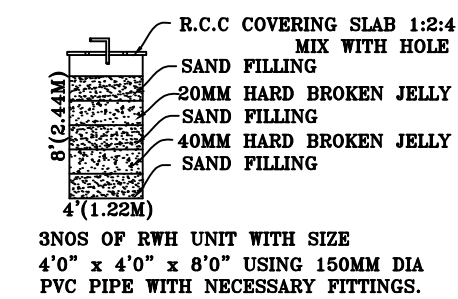
RAIN WATER HARVEST UNIT
