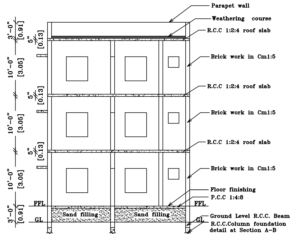
SECTION ON 'SD'
