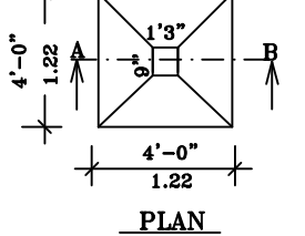
COLUMN DETAILS
