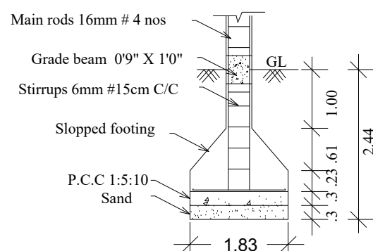
COLUMN DETAIL
