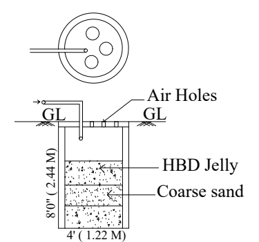
WASTE WATER RECYCLE UNIT
