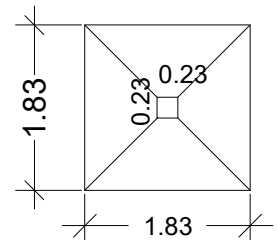
FOOTING
