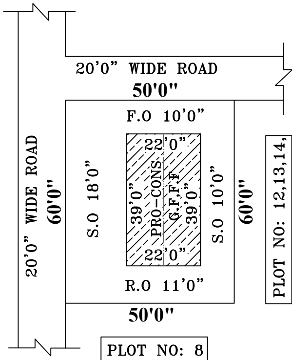
SITE PLAN SCALE: 1INCH=33FEET
