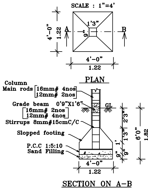
COLUMN DETAILS
