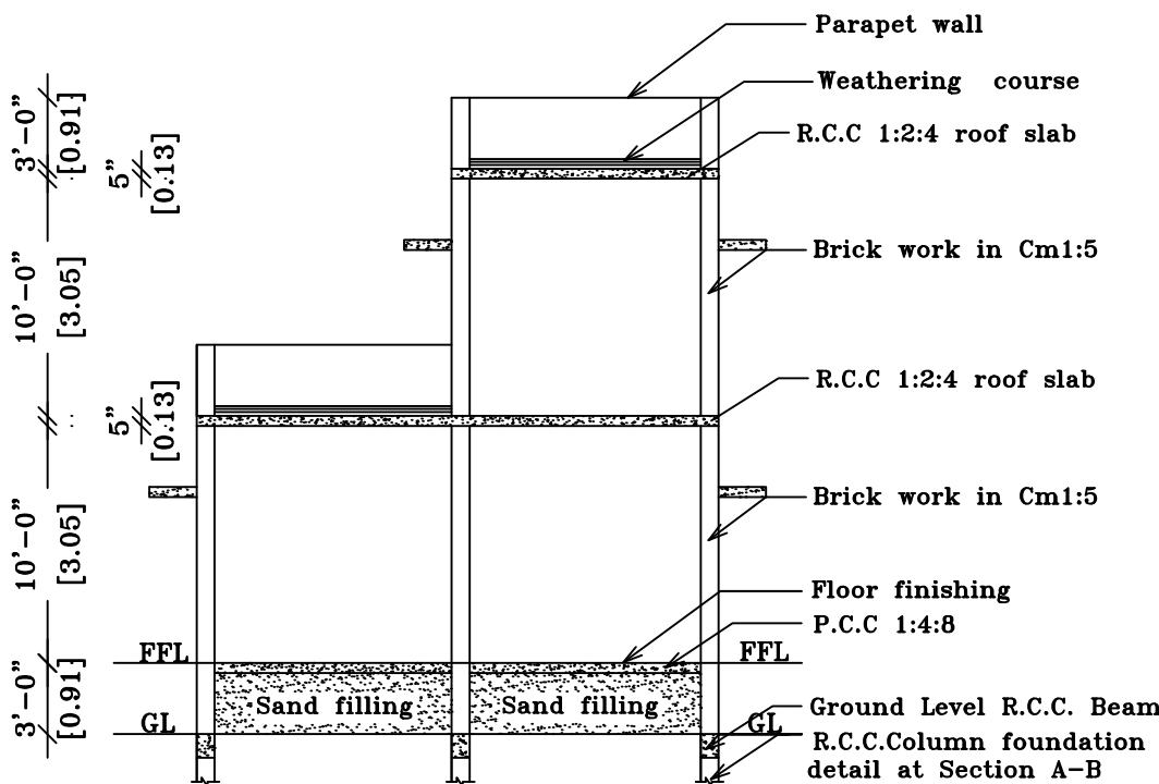
SECTION ON 'SK'
