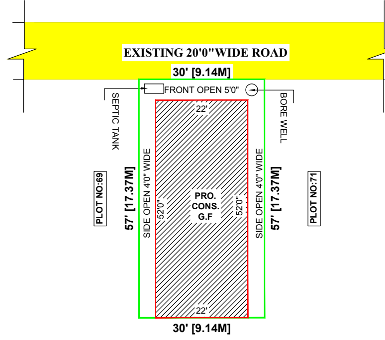
SITE PLAN
