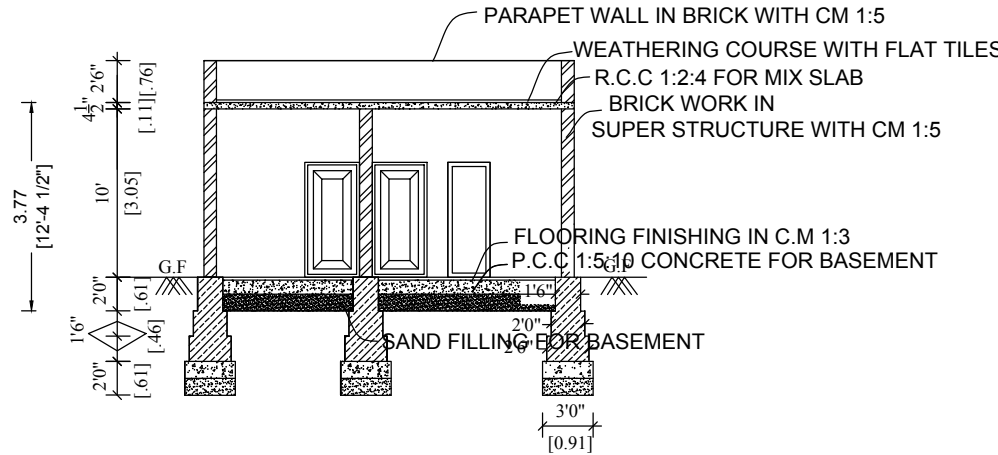
SECTION NO R-S
