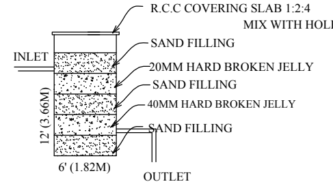
Waste Water Recycle Unit Not To Scale
