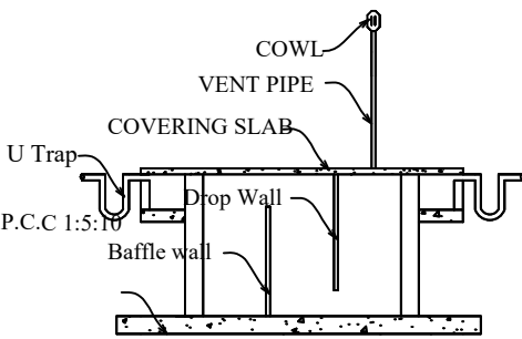
SECTION ON JS1
