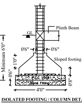
ISOLATED FOOTING / COLUMN DETAIL
