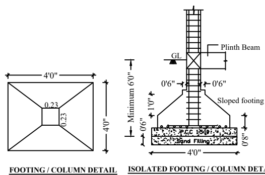
FOOTING / COLUMN DETAIL
