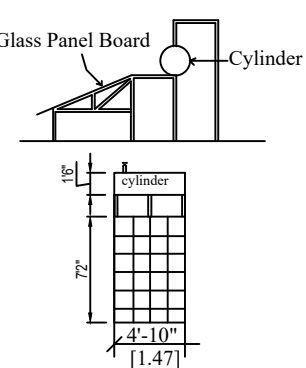
SOLAR ENERGY SYSTEM
