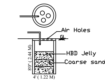
RAIN WATER HARVESTING TANK DETAIL
