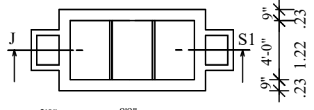
PLAN
