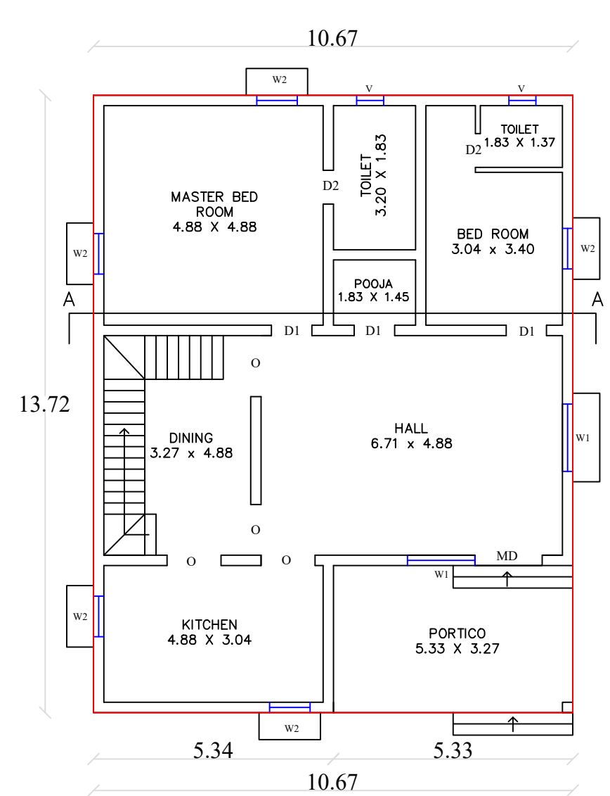
GR PLAN
