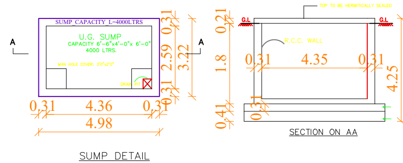
SUMP DETAIL
