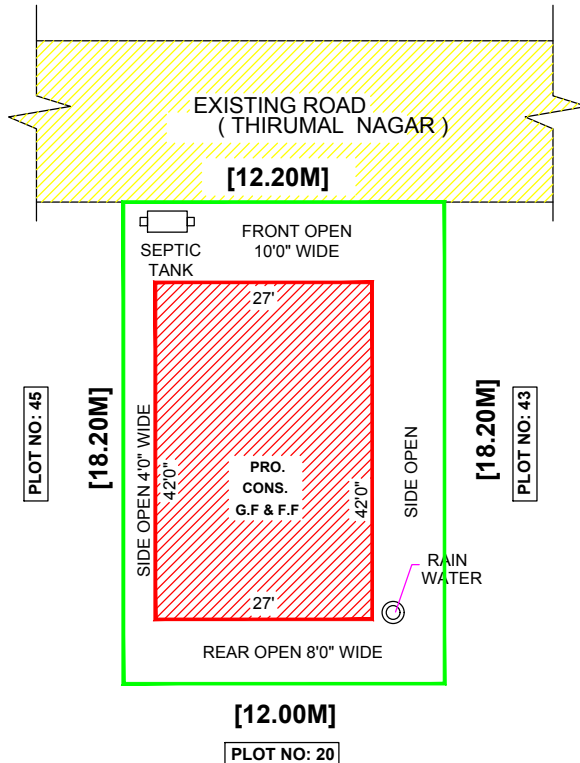
SITE PLAN SCALE - 1CM = 2M
