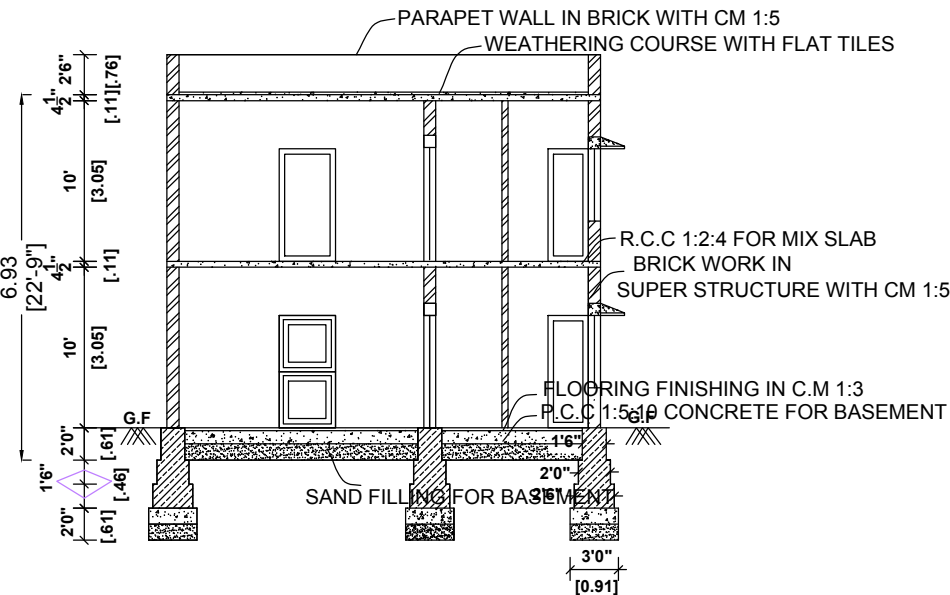
SECTION NO R-S
