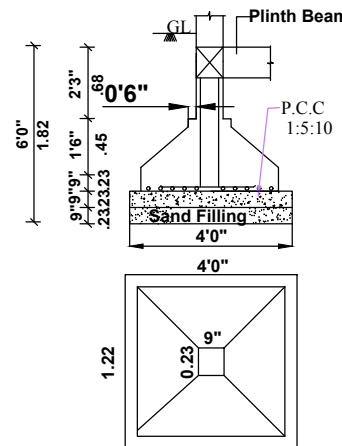
COLUMN DETAIL NOT TO SCALE
