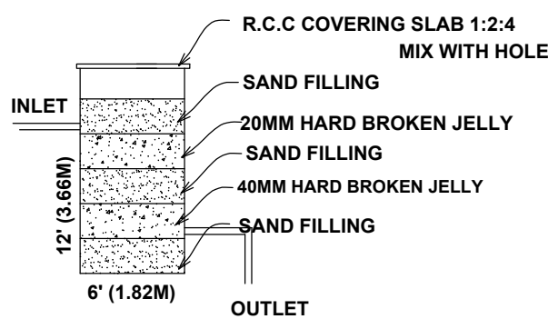
Waste Water Recycle Unit Not To Scale
