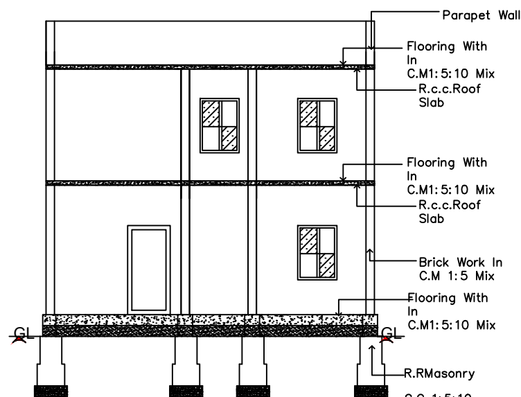
SECTION @ AA' FOUNDATION DETAIL DESIGNED
