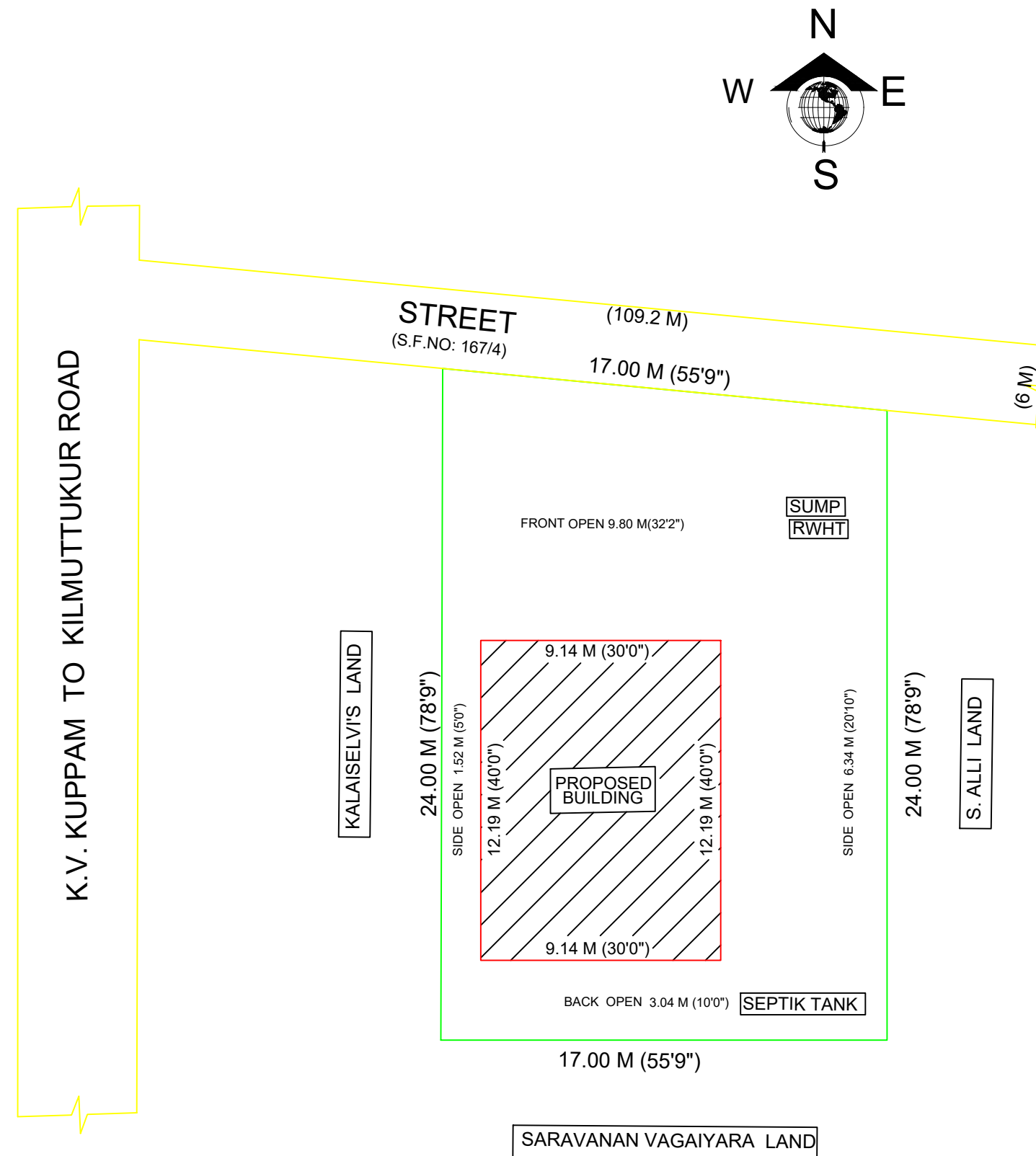
SITE PLAN TO SCALE
