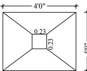
FOOTING / COLUMN DETAIL
