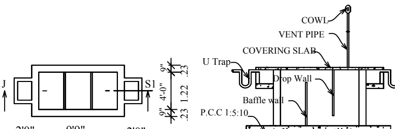
SECTION ON JS1
