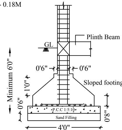
ISOLATED FOOTING / COLUMN DETAIL
