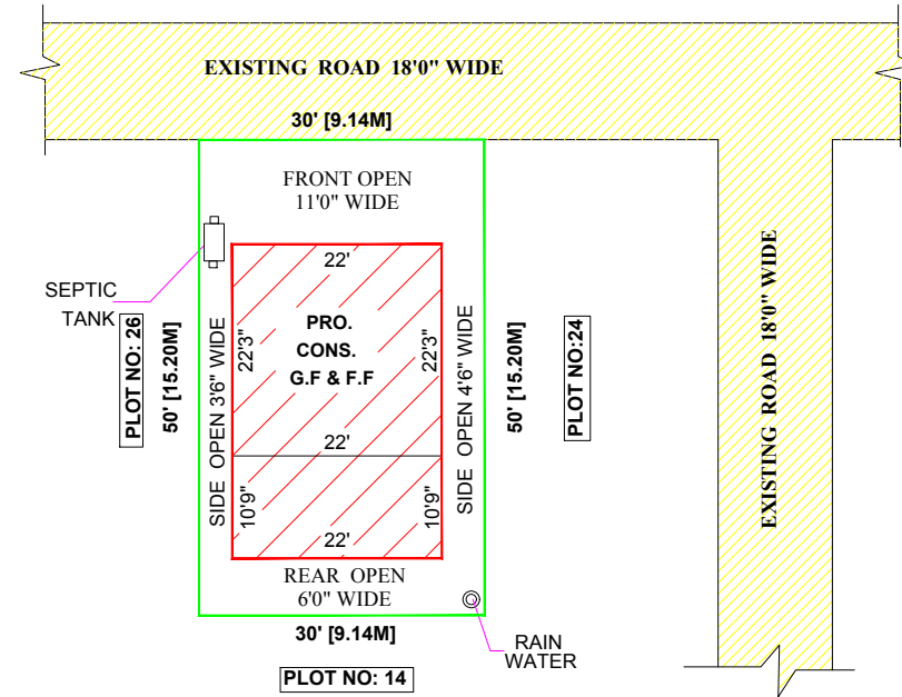
SITE PLAN SCALE - 1CM = 2M
