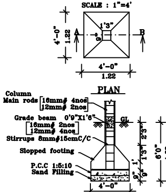
SECTION ON A-B
