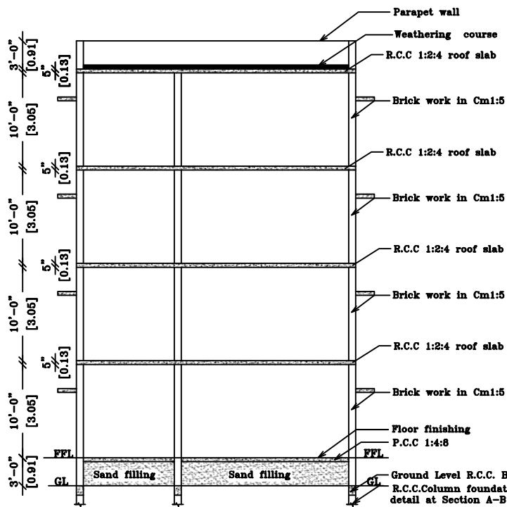
SECTION ON 'SA'
