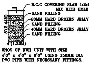
RAIN WATER HARVEST UNIT
