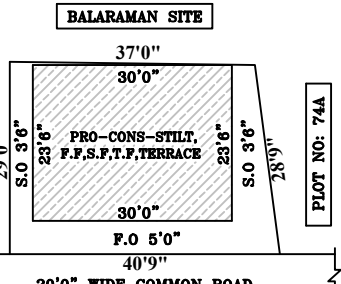
SITE PLAN SCALE: 1INCH=33FEET
