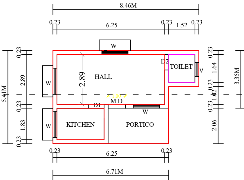
PRO.. ADDL..GROUND FLOOR PLAN
