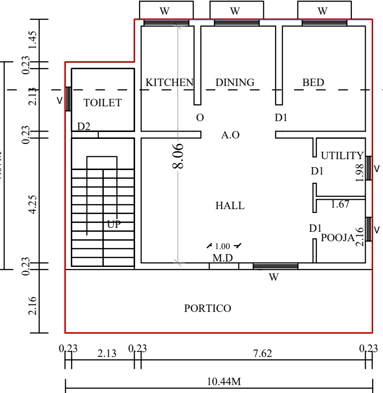
EXI.. GROUND FLOOR PLAN
