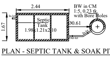
PLAN - SEPTIC TANK & SOAK PIT
