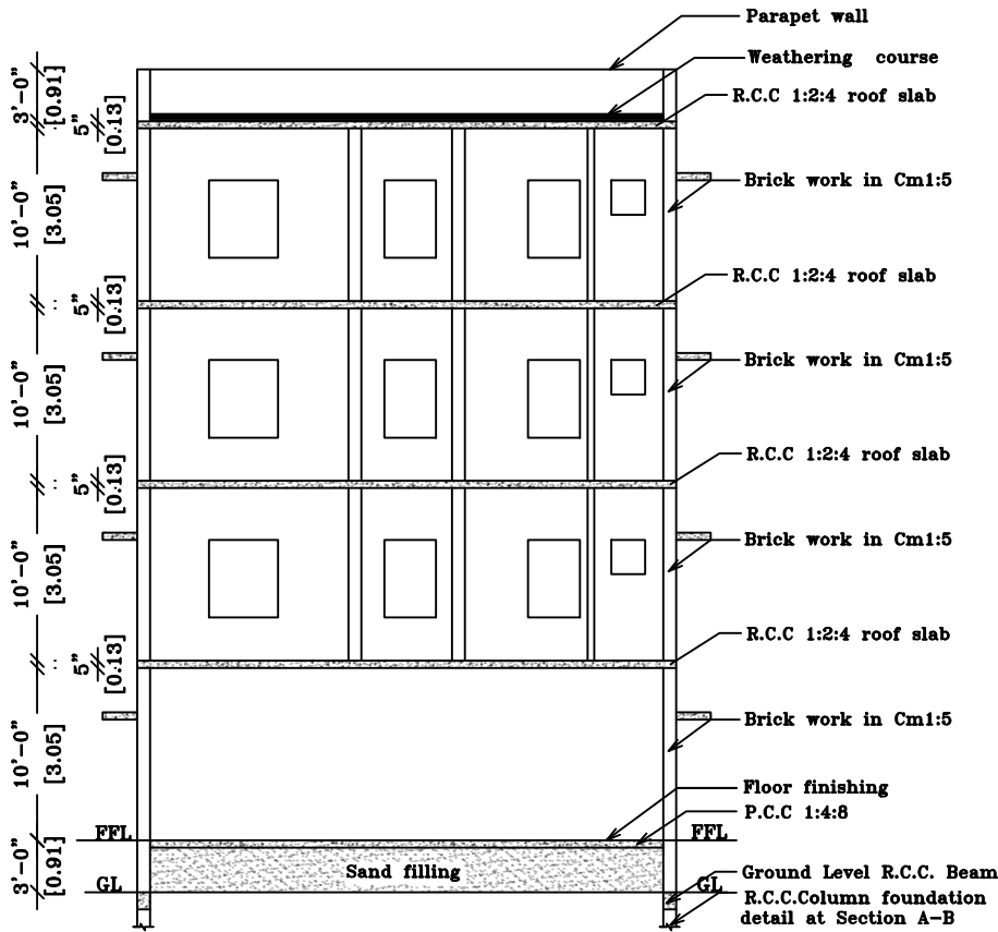
SECTION ON 'A'
