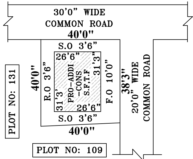
SITE PLAN
