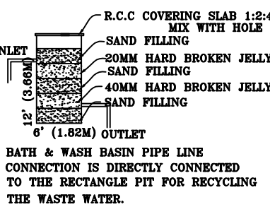
WASTE WATER RECYCLE UNIT
