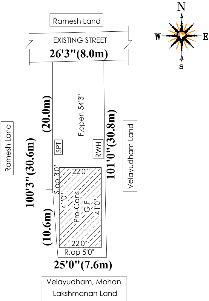
SITE PLAN SCALE:1INCH = 33FEET
