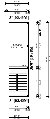
ST FLOOR PLAN.
