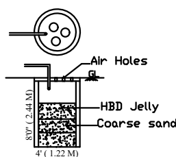
RAIN WATER HARVESTING TANK DETAIL
