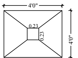
FOOTING / COLUMN DETAIL
