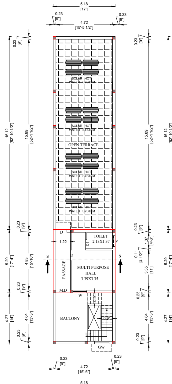
PRO., ADDITIONAL SECOND FLOOR PLAN
