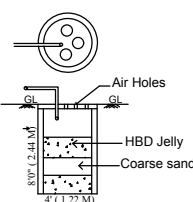
WASTE WATER RECYCLE UNIT
