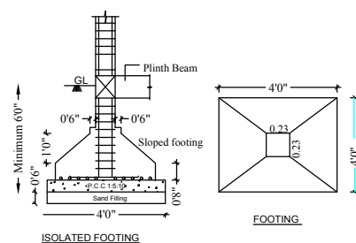
COLUMN DETAILS
