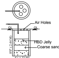
RAIN WATER HARVESTING TANK DETAIL
