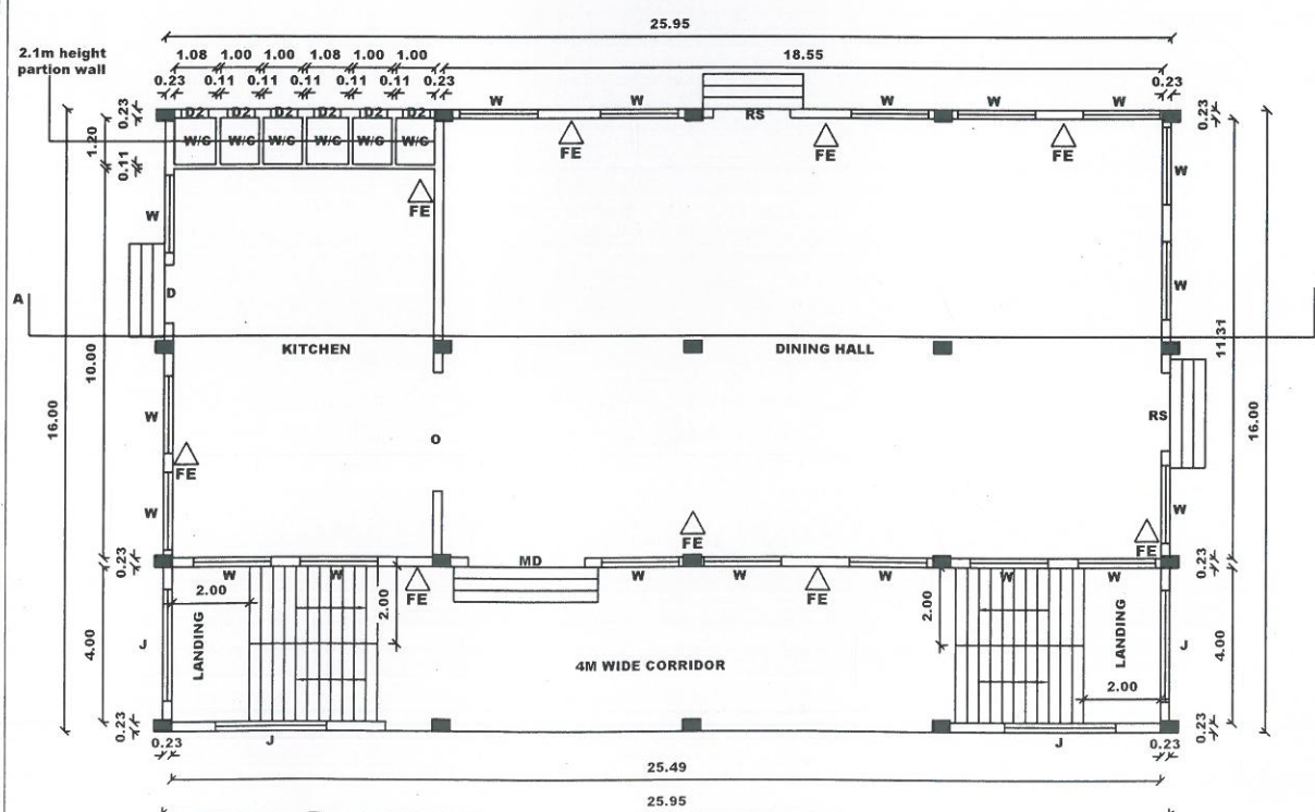
GROUND FLOOR
