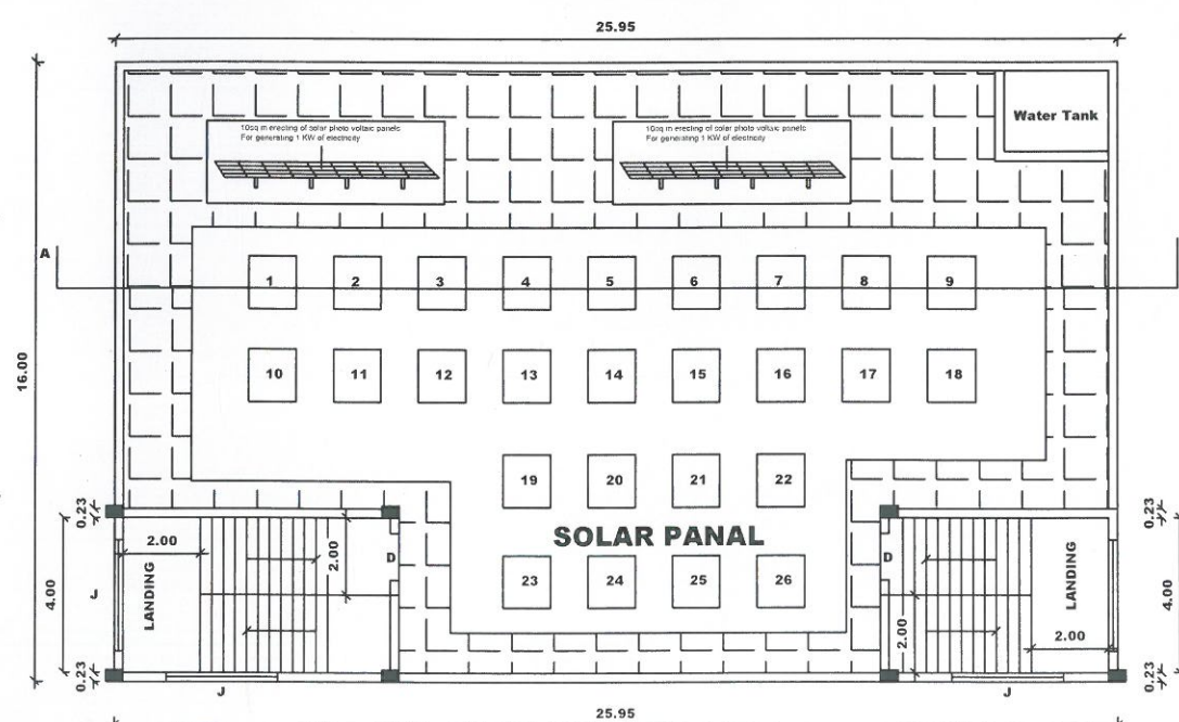
TERRACE FLOOR
