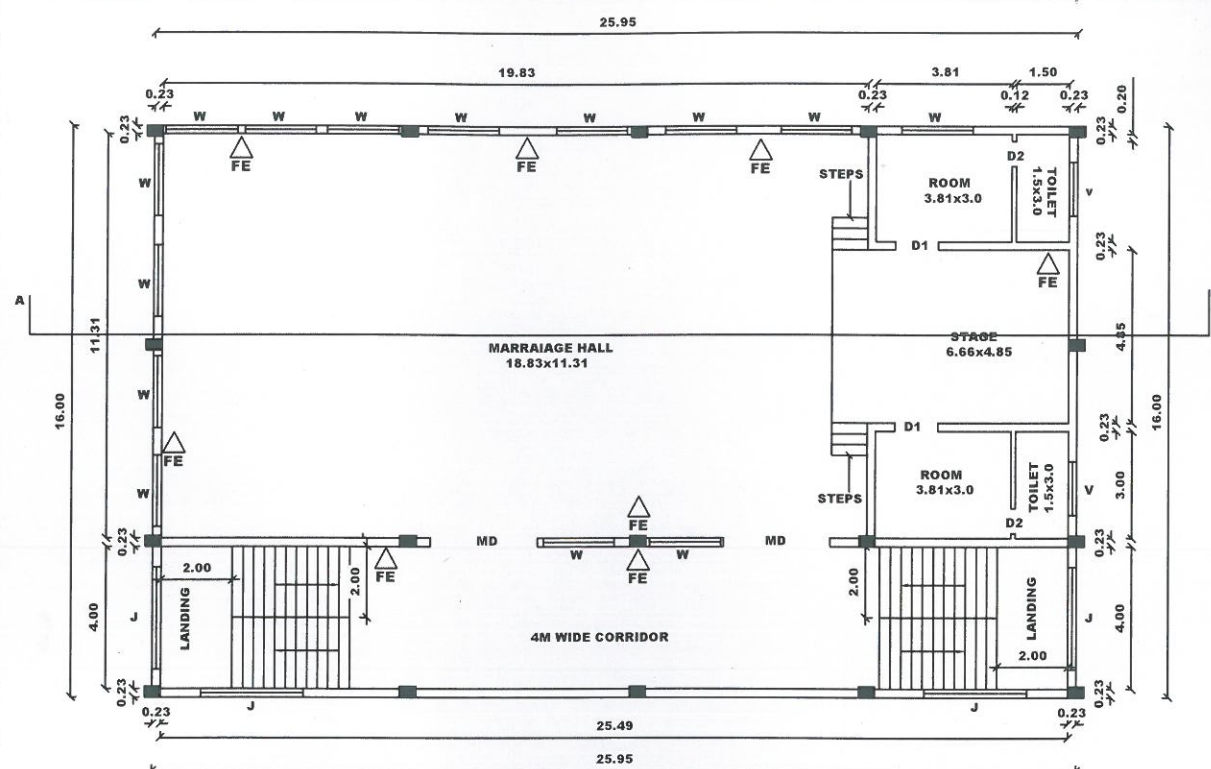
FIRST FLOOR
