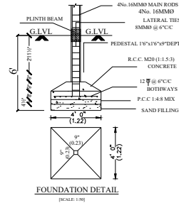
FOUNDATION DETAIL
