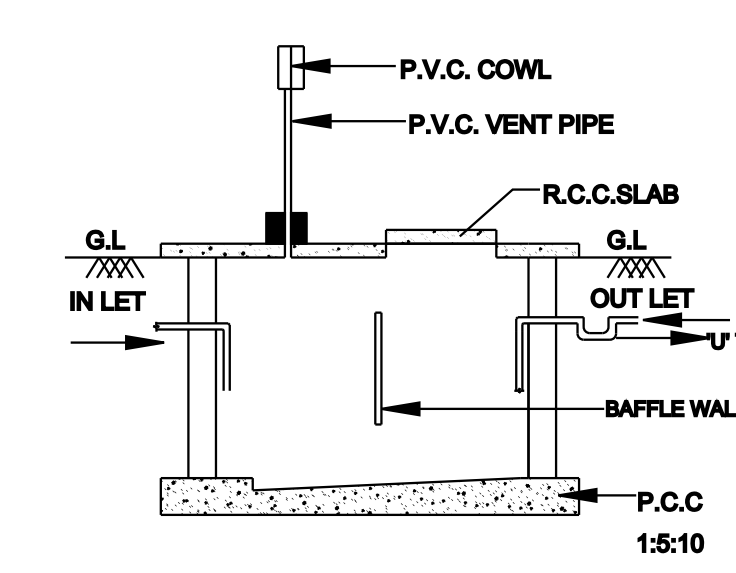
SEC. OF SEPTIC TANK
