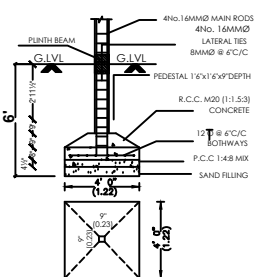
FOUNDATION DETAIL
