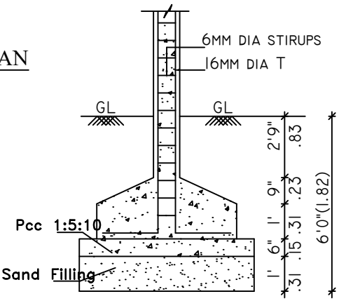
COLUMN FOUNDATION DETAIL SCALE 1"=4'0"(1:50)
