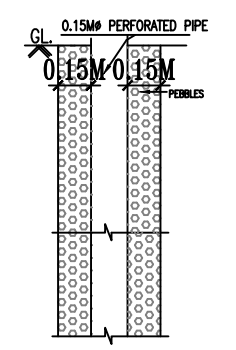
PLAN BORE WELL "nts"
