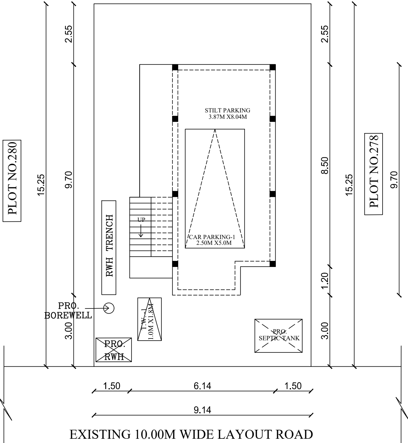
PROPOSED SITE CUM STILT FLOOR PLAN
