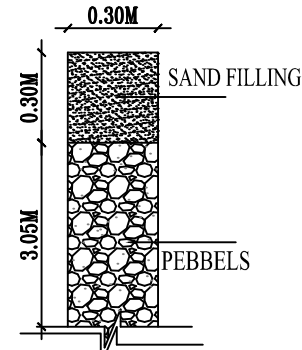
PERCOLATION PIT
