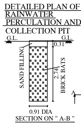
SECTION ON "A-B"
