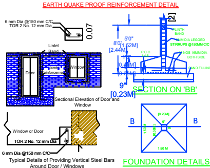
FOUNDATION DETAILS
