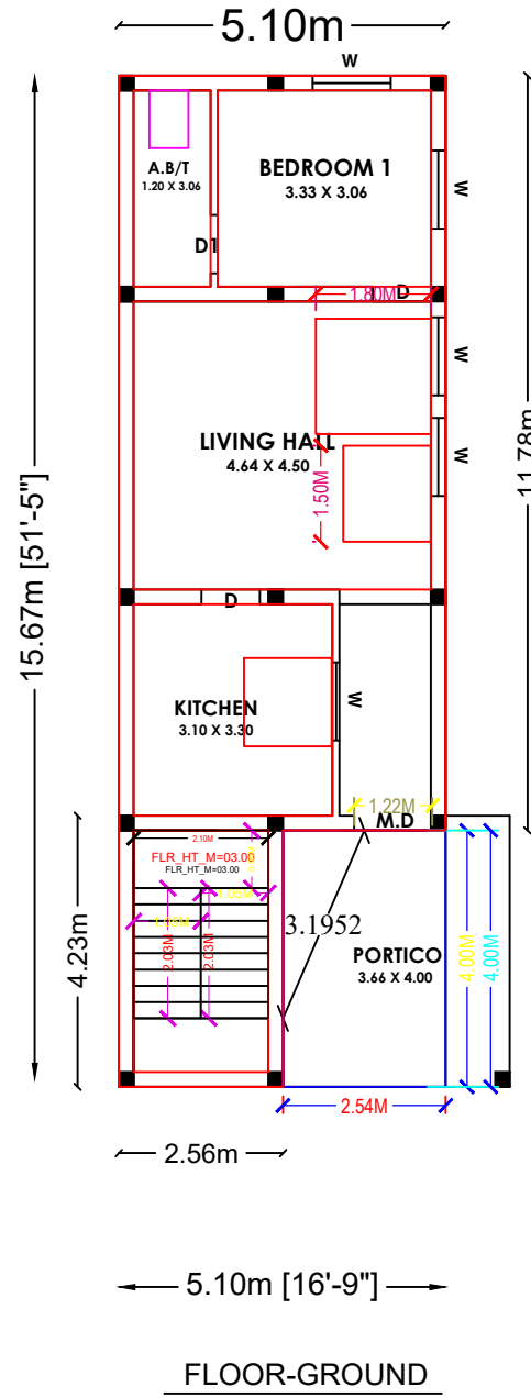
FLOOR-GROUND
