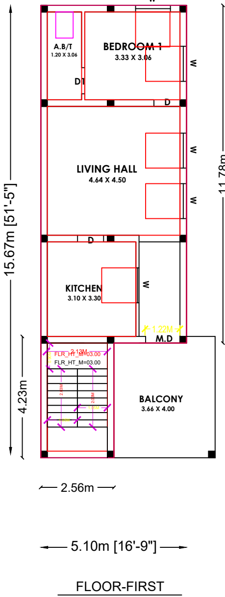
FLOOR-FIRST
