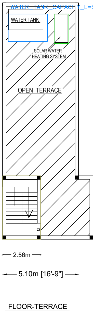
FLOOR-TERRACE
