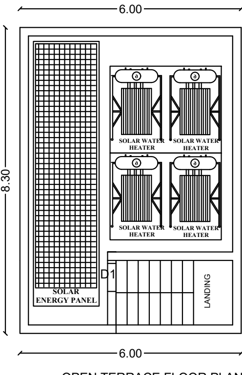
OPEN TERRACE FLOOR PLAN
