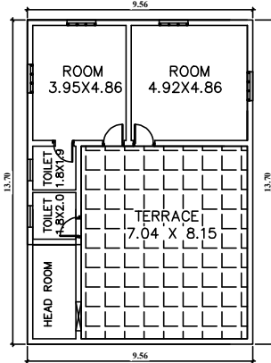
PROPOSED TERRACE FLOOR PLAN
