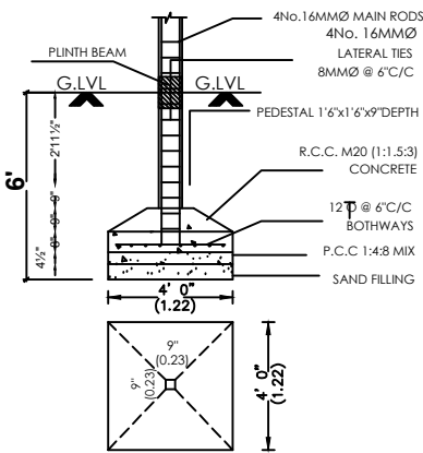
FOUNDATION DETAIL
