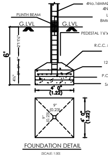
FOUNDATION DETAIL (SCALE 1:30)
