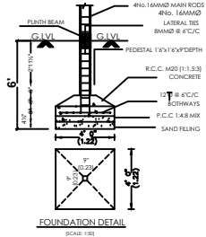
FOUNDATION DETAIL (SCALE: 1:50)
