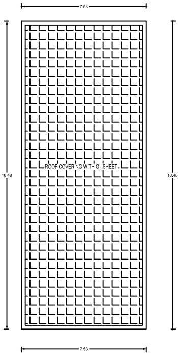
TERRACE PLAN
