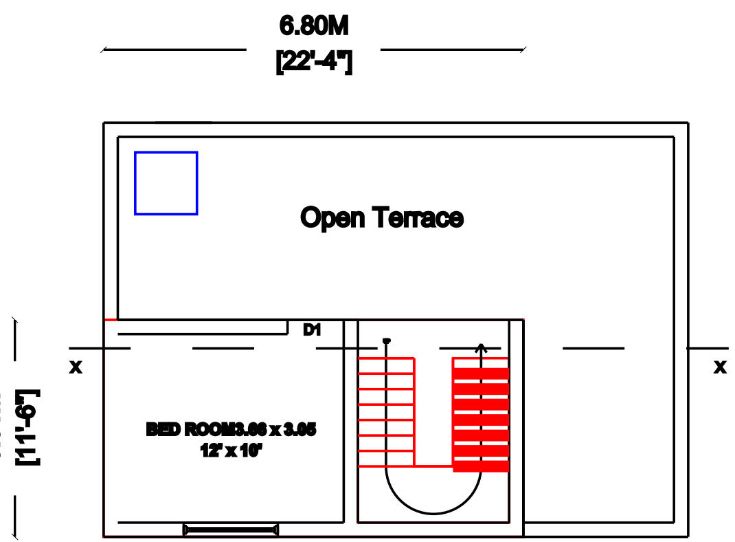
FIRST FLOOR / TERRACE FLOOR PLAN
