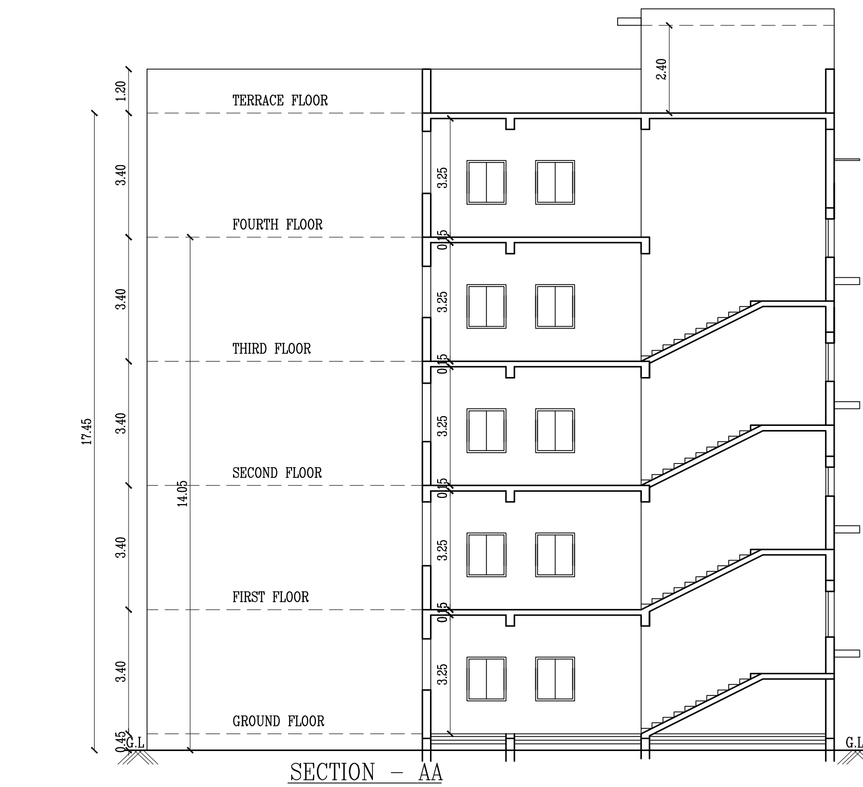
SECTION - AA
