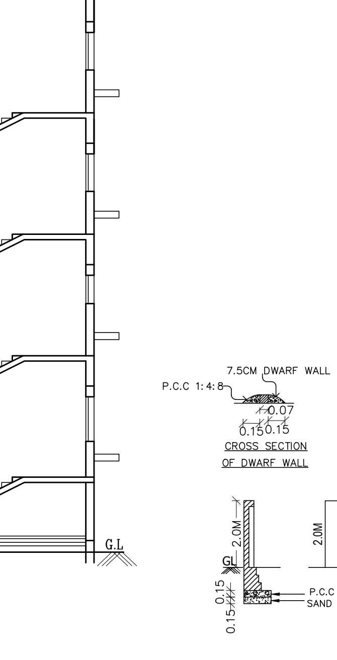
CROSS-SECTION OF DWARF WALL
