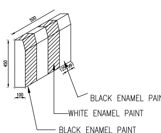
TYPICAL KERB WALL SIDE VIEW
