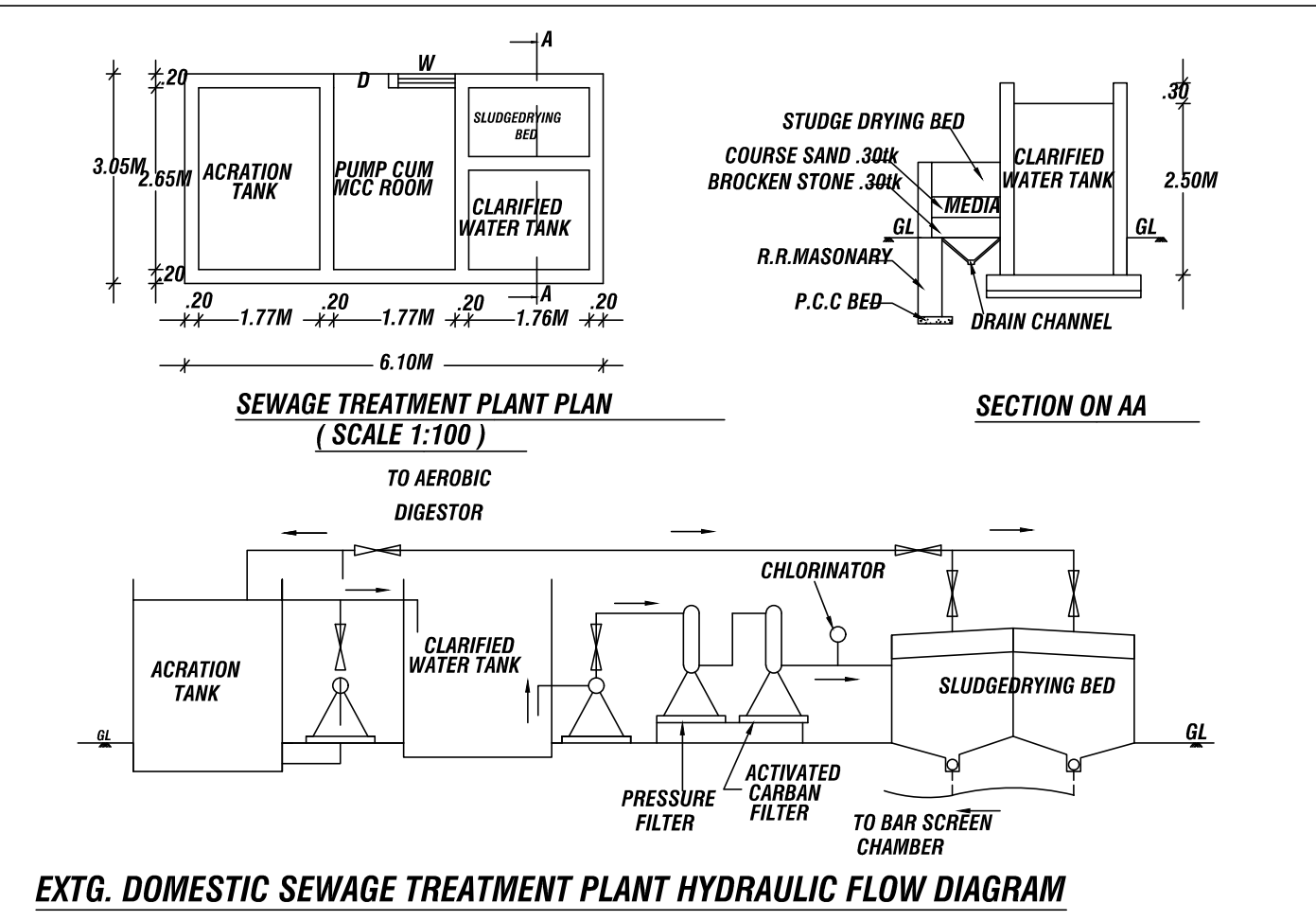
EXTG. DOMESTIC SEWAGE TREATMENT PLANT HYDRAULIC FLOW DIAGRAM
