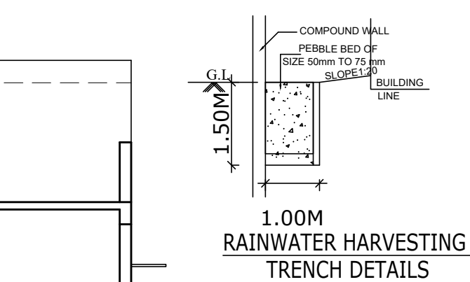
1.00M RAINWATER HARVESTING TRENCH DETAILS
