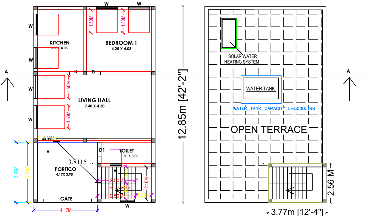
TERRACE PLAN
