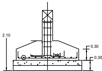
section A-A Typical section through footing.
