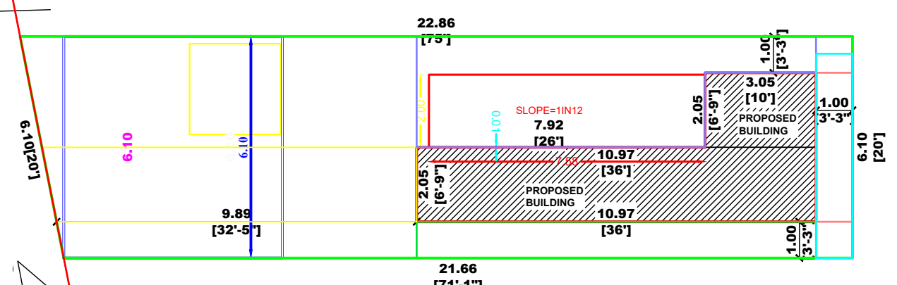
SITE PLAN
