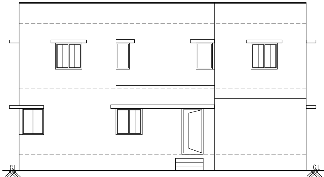
FRONT ELEVATION
