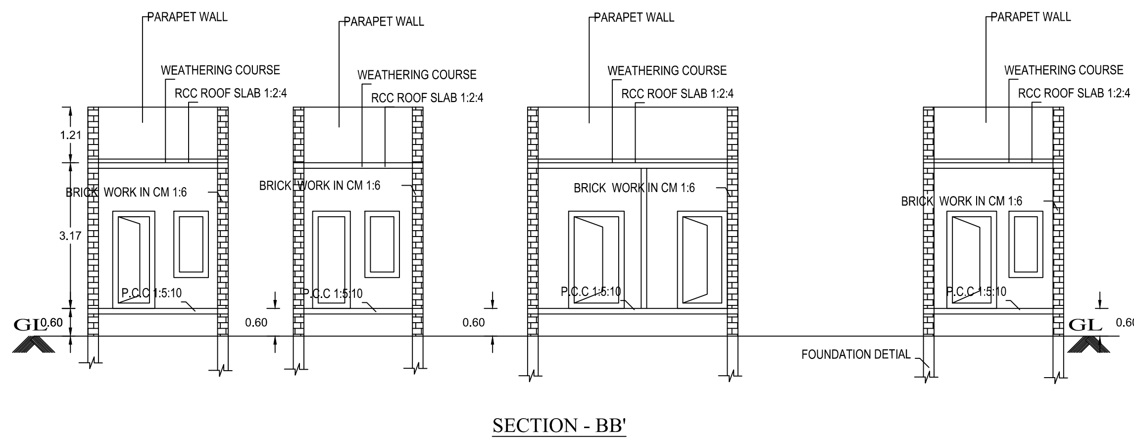
SECTION - BB'
