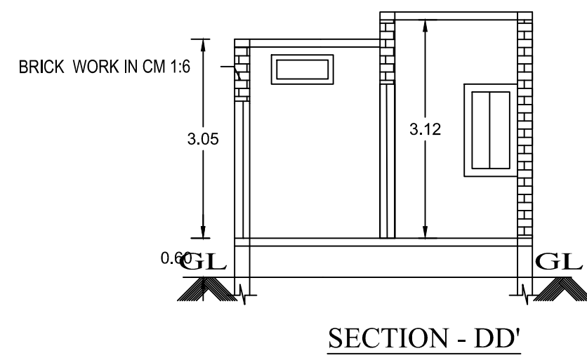
SECTION - DD'
