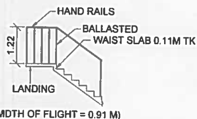
STAIRCASE DETAIL
