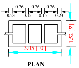
SEPTIC TANK DETAILS SCALE-1:100
