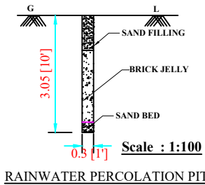
RAINWATER HARVESTING SYSTEM
