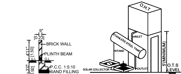
SOLAR WATER HEATING SYSTEM
