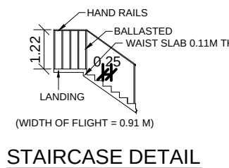
STAIRCASE DETAIL
